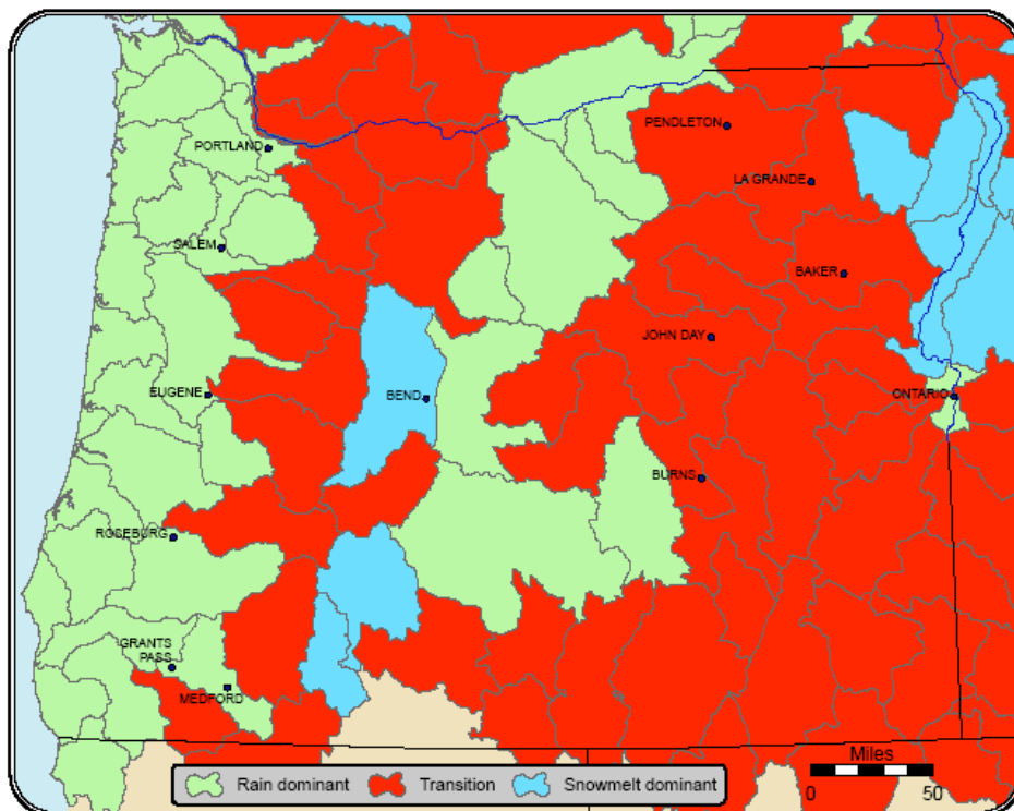
Figure 25. Classification of Oregon HUC4 watersheds as snow dominated, rain dominated, or transition. The classification was calculated as the long-term average of the peak SWE divided by the long-term average of total cool season (October through March). This figure (reprinted with permission) was originally produced by Dr. Alan F. Hamlet of the CSES Climate Impacts Group and the Department of Civil and Environmental Engineering at the University of Washington as part of a report for the Climate Leadership Initiative, University of Oregon (Hamlet 2007).
