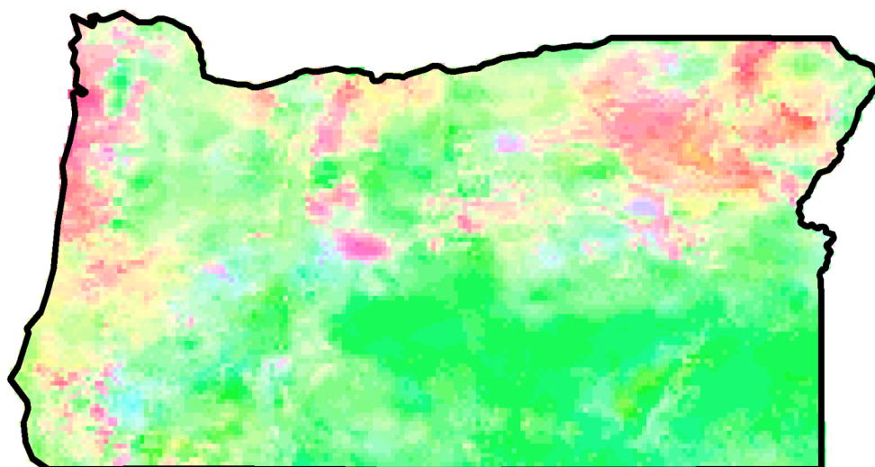
Figure 17. Trends in both annual minimum temperatures and annual precipitation from 1895-2006. The colors represent different combinations of directional changes in precipitation and temperature. The intensity of the color depicts the magnitudes of the trends. Refer to Figures 4 and 11 for descriptions of the contributing analyses.
